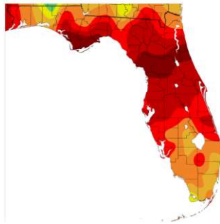
Departure from Normal Precipitation (in) 1/1/2020 - 3/31/2020
