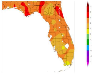
Departure from Normal Temperature (F) 1/1/2020 - 3/31/2020
